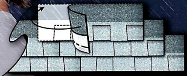
THE 2 SEALANT BANDS ADHERE TO THE PREVIOUS SHINGLE ROW, PROVIDING DOUBLE PROTECTION AGAINST THE ELEMENTS.
